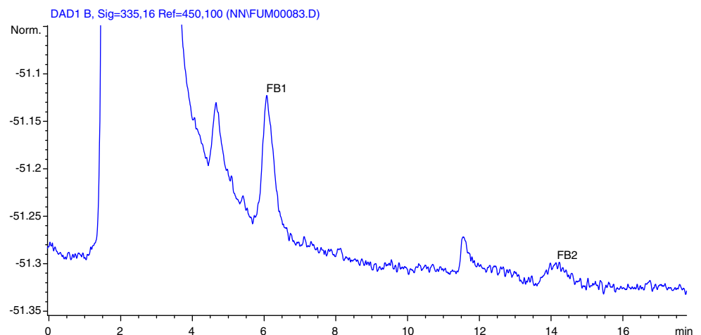
Fig. 2 Naturally contaminated sample with 968 \mu\text{g}/\text{kg} and 321 \mu\text{g}/\text{kg} levels of \text{FB}_1 and \text{FB}_2 , respectively. Analysis done by HPLC-DAD
