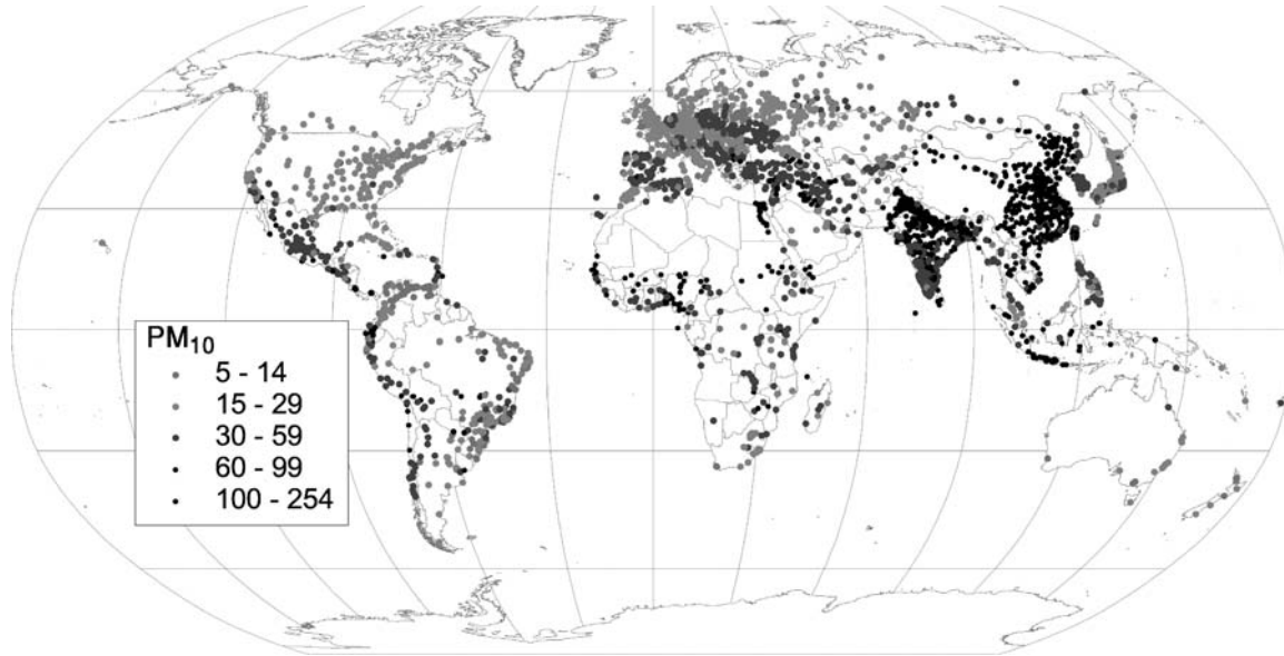
Figure 3 Estimated annual average concentrations of PM 10 (particulates below 10 microns in aerodynamic diameter) in cities with populations of 100,000 or more and national capitals in 2000. [Figure from (18).]
